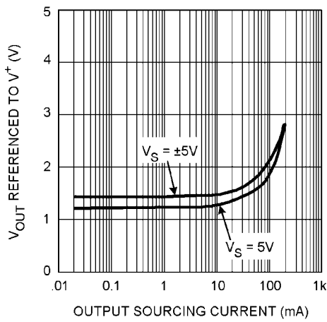
Output Sourcing Current
