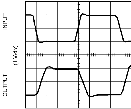
Inverting Large Signal Pulse Response ( V_S = \pm 5V )
