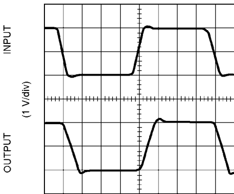
Non-Inverting Large Signal Pulse Response ( V_S = \pm 5V )
