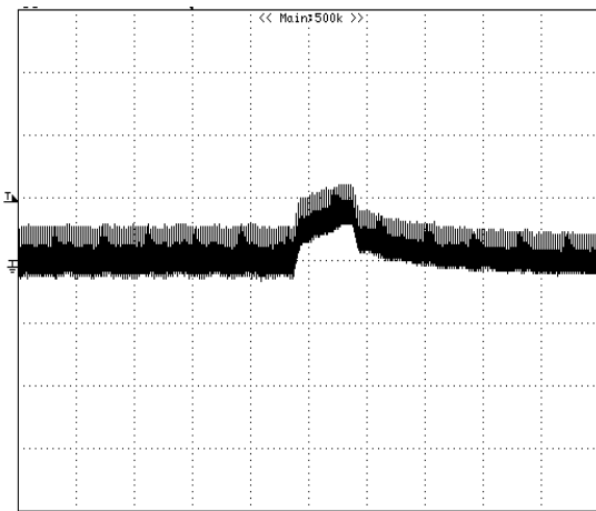
Figure 8: Output voltage response to step-change in load current (75%-50% of I_{o, \max} ; di/dt = 0.1A/\mu s ). Load cap: 10\mu F , tantalum capacitor and 1\mu F ceramic capacitor. Trace: V_{out} (20mV/div, 100us/div), Scope measurement should be made using a BNC cable (length shorter than 20 inches). Position the load between 51 mm to 76 mm (2 inches to 3 inches) from the module..
