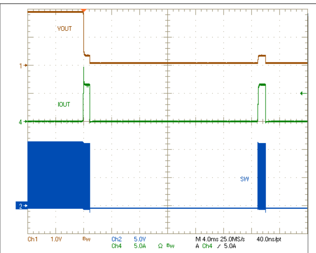
Figure 2-18. TPS54424EVM-779 Hiccup Mode Start
