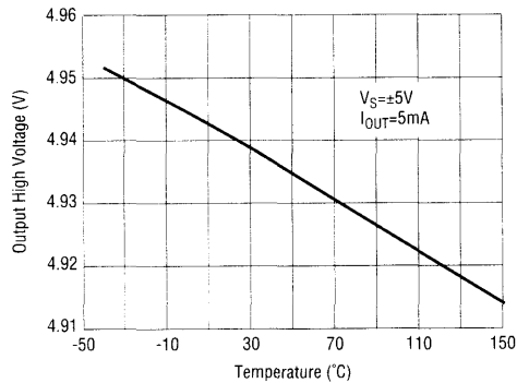
Output High Voltage vs Temperature
