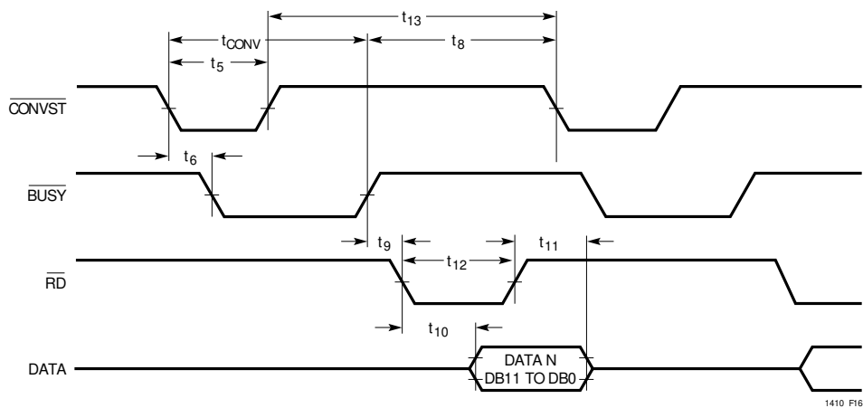
Figure 16. Mode 2. CONVST Starts a Conversion. Data is Read by RD
