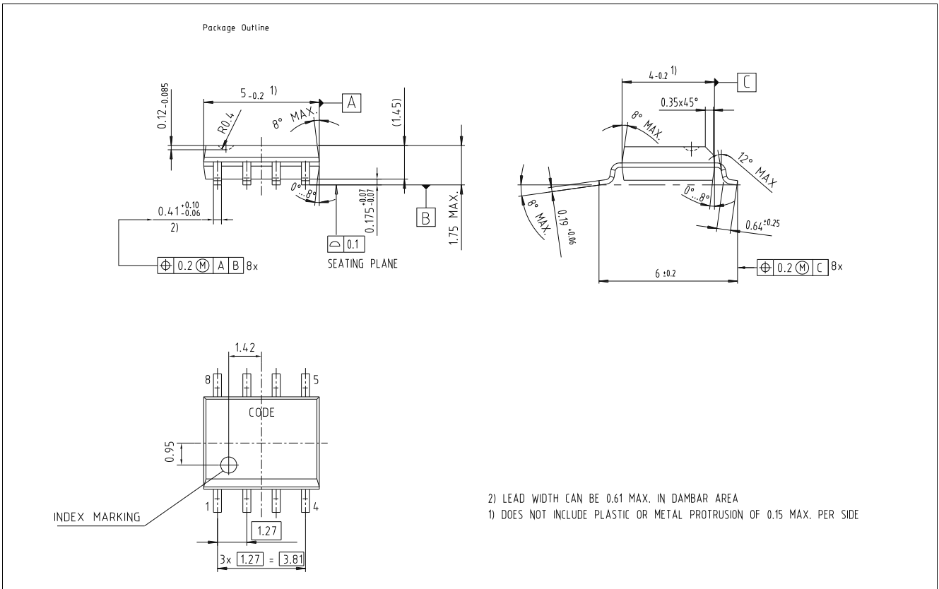
Figure 12 Package outline
