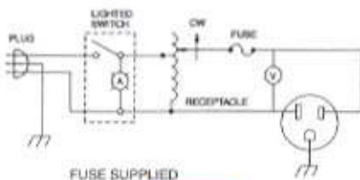
FUSE SUPPLIED
