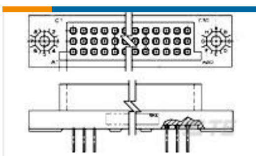
TE Part #448005-1 3 ROW BOX RECP 180 POS 100C/L
