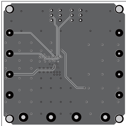
Figure 3—Inner Layer 2
