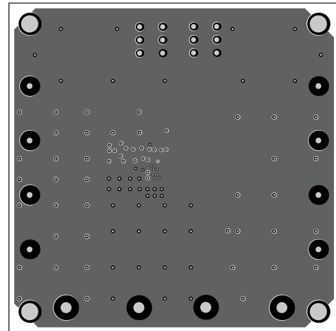
Figure 2—Inner Layer 1
