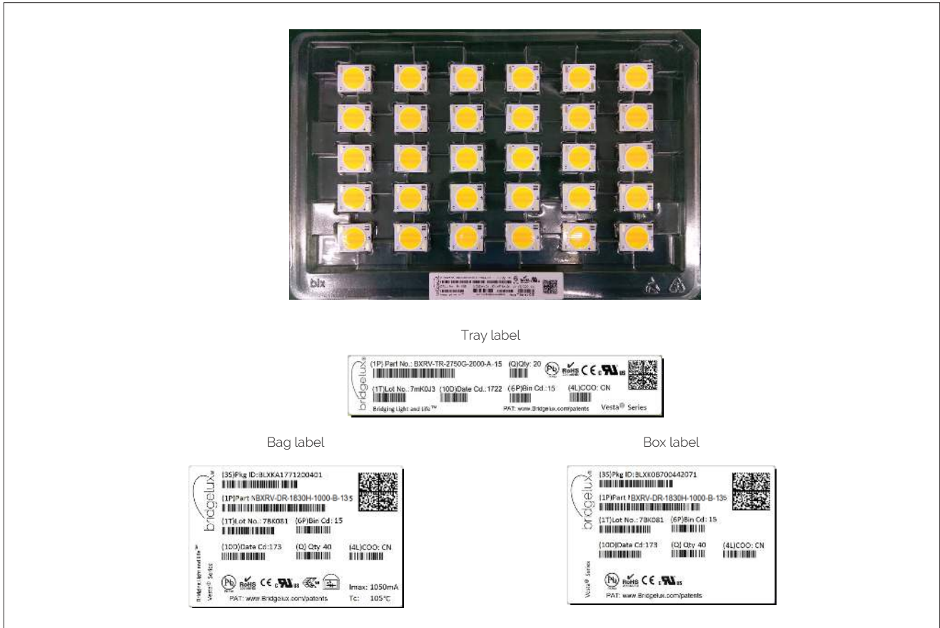
Figure 21: Vesta Series Dim-To-Warm 13mm and 15mm Packaging and Labeling
