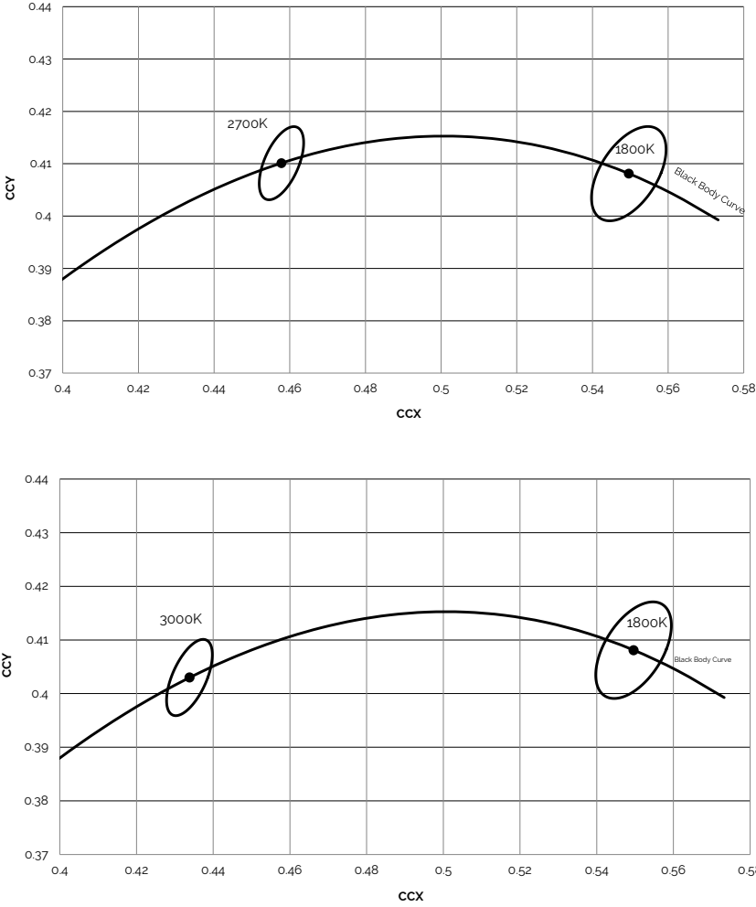
Figure 20: Graph of Warm White Test Bins in xy Color Space
