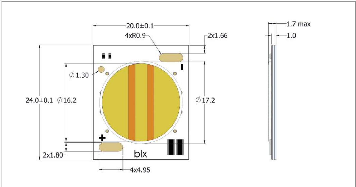
Figure 19: Drawing for Vesta Series Dim-To-Warm 15mm Array
