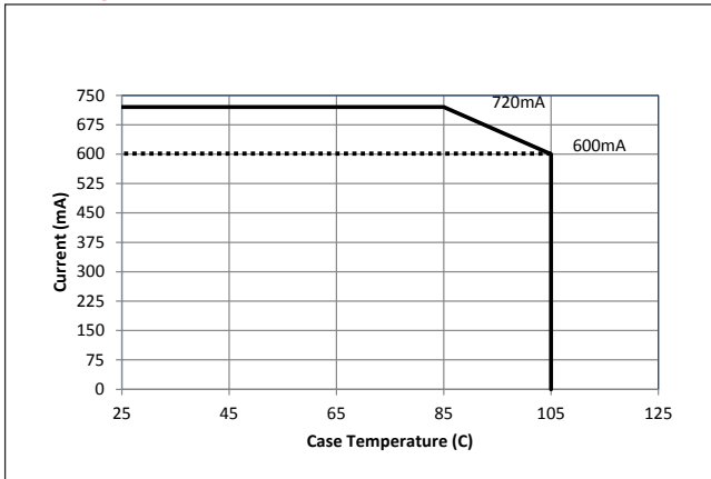
Figure 13: Vesta Dim-to-Warm 13mm 20W Derating Curve
