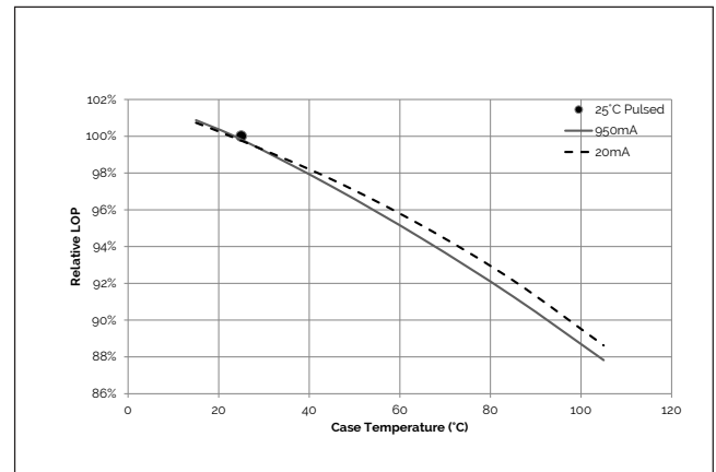
Figure 6: Vesta Dim-to-Warm 15mm 33W Relative Flux vs. Case Temperature
