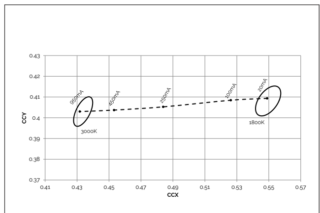
Figure 12: Vesta Dim-to-Warm 15mm 33W Color Shift vs. Forward Current 3000K-1800K
