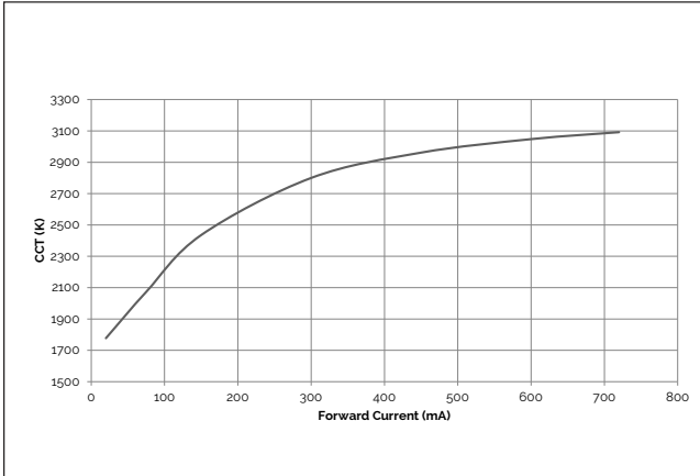
Figure 7: Vesta Dim-to-Warm 13mm 20W CCT vs. Forward Current
