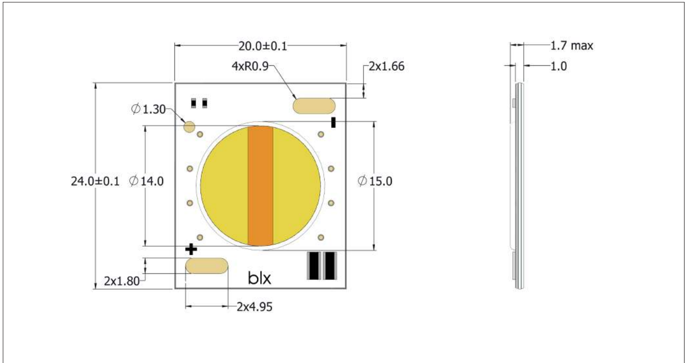
Figure 18: Drawing for Vesta Series Dim-To-Warm 13mm Array
