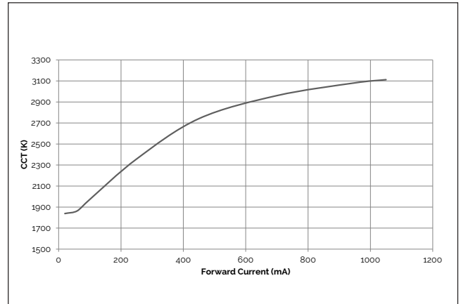
Figure 8: Vesta Dim-to-Warm 15mm 33W CCT vs. Forward Current
