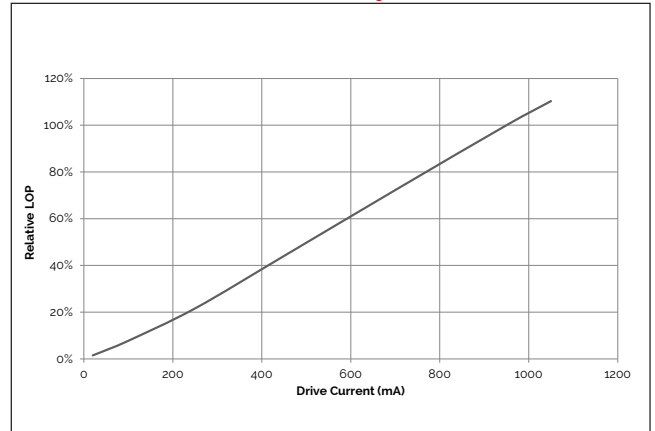
Figure 4: Vesta Dim-to-Warm 15mm 33W Relative LOP vs. Drive Current, T_c = 25^\circ\text{C}
