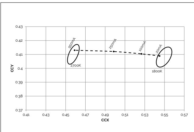
Figure 11: Vesta Dim-to-Warm 15mm 33W Color Shift vs. Forward Current 2700K-1800K
