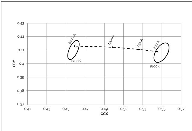
Figure 9: Vesta Dim-to-Warm 13mm 20W Color Shift vs. Forward Current 2700K-1800K
