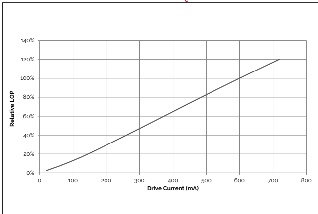
Figure 3: Vesta Dim-to-Warm 13mm 20W Relative LOP vs. Drive Current, T_c = 25^\circ\text{C}
