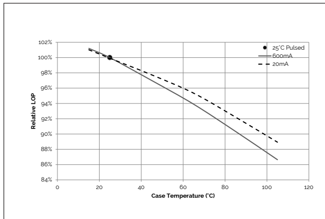
Figure 5: Vesta Dim-to-Warm 13mm 20W Relative Flux vs. Case Temperature
