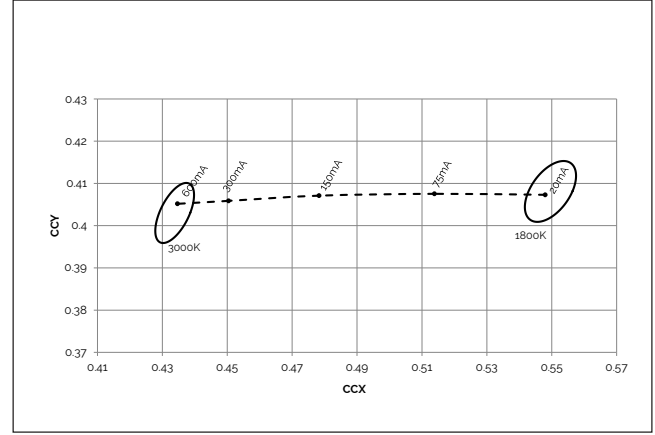
Figure 10: Vesta Dim-to-Warm 13mm 20W Color Shift vs. Forward Current 3000K - 1800K
