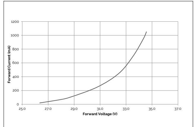
Figure 2: Vesta Dim-to-Warm 15mm 33W Forward Voltage vs. Forward Current, T_c = 25^\circ\text{C}
