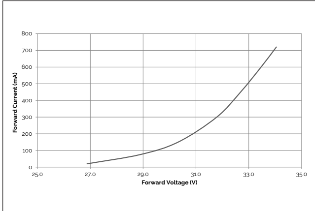
Figure 1: Vesta Dim-to-Warm 13mm 20W Forward Voltage vs. Forward Current, T_c = 25^\circ\text{C}
