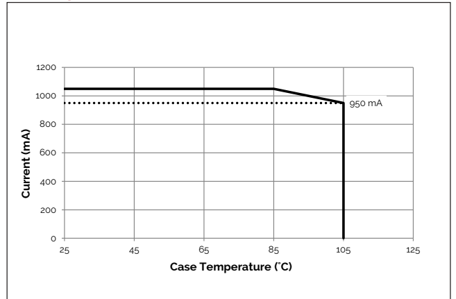
Figure 14: Vesta Dim-to-Warm 15mm 33W Derating Curve
