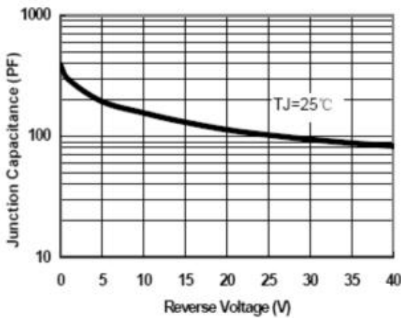
Fig.1-Typical Junction Capacitance
