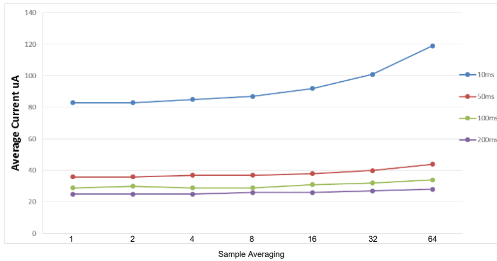
Figure 37-8. 1 Sensor/PTC_GCLK = 2 MHz/FREQ_MODE_HOP
