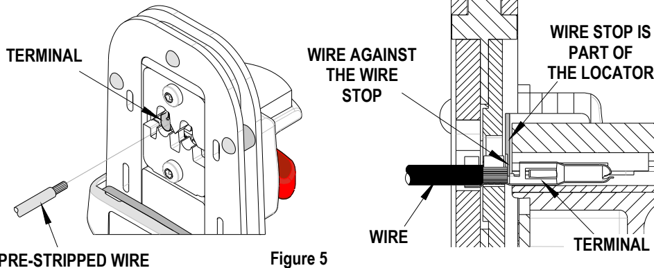
PRE-STRIPPED WIRE
