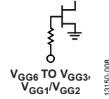
Figure 8. V_{GG6} to V_{GG3} , V_{GG1}/V_{GG2} Interface
