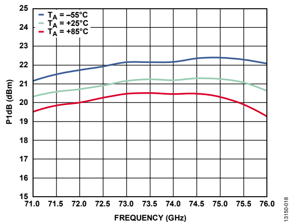
Figure 19. Output P1dB vs. Frequency at Various Temperatures, V_{CTL1}/V_{CTL2} = -5 V
