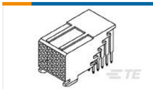
TE Part #5106081-1 Hard Metric Male Connector: Traditional Backplane, Mezzanine, 2mm
