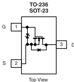
SQ7002K (8K)* * Marking Code 8K
