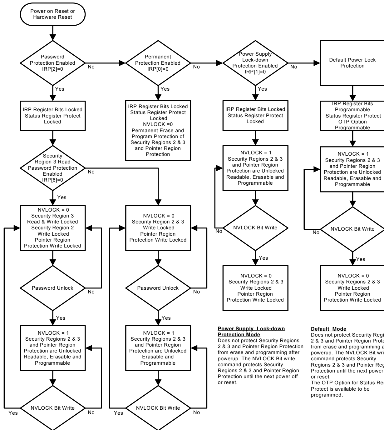
Figure 8.3 Permanent, Password and Power Supply Lock-down Protection Overview
