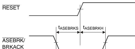
Figure 23.66 \overline{RESET} Hold Timing
