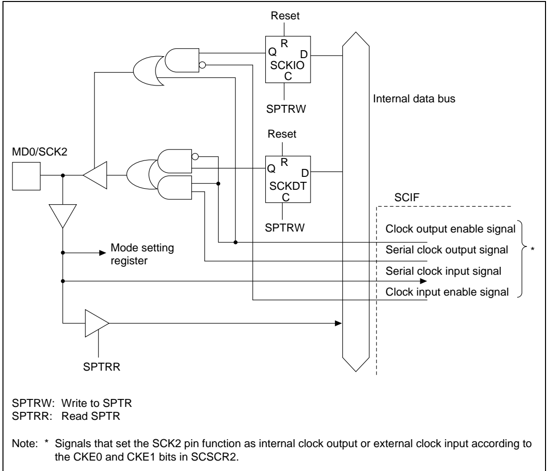
Figure 18.8 MD0/SCK2 Pin
