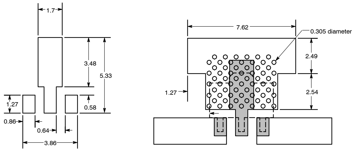
Recommended Solder Stencil
