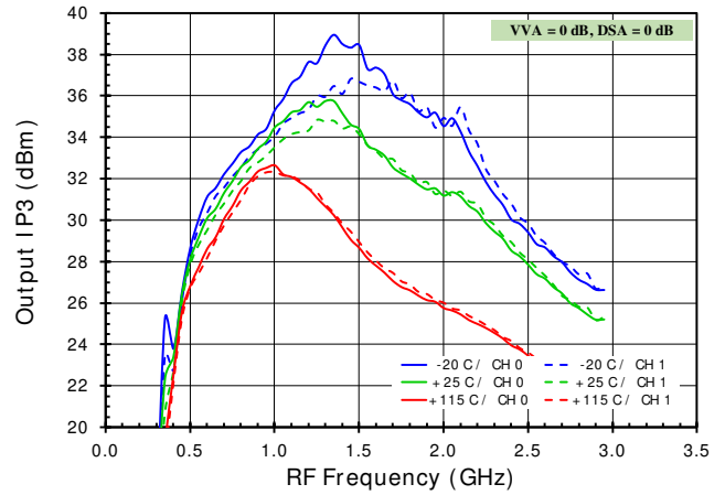
Figure 35. OIP3 versus Frequency (+3.3V)
