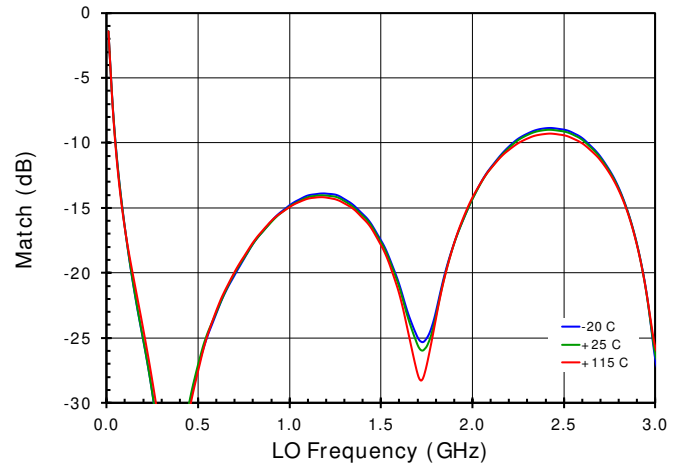
Figure 6. LO Differential Output Return Loss
