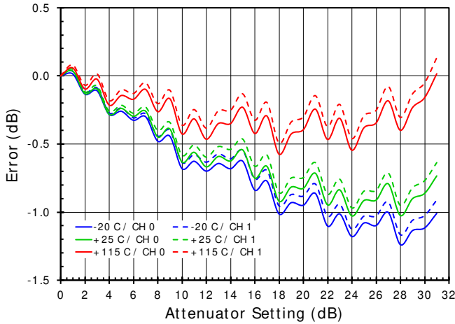
Figure 18. Step Error versus DSA (+3.3V)
