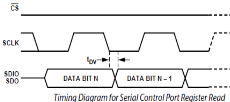
Figure 96. Serial Timing Diagram for Multiple Bits
