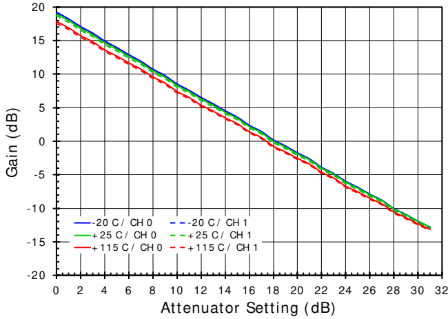
Figure 16. Gain Accuracy versus DSA (+3.3V)
