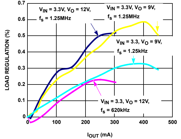
FIGURE 5. LOAD REGULATION vs I OUT
