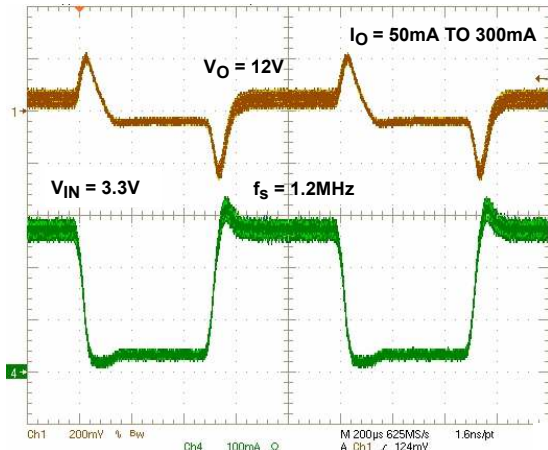
FIGURE 8. TRANSIENT RESPONSE
