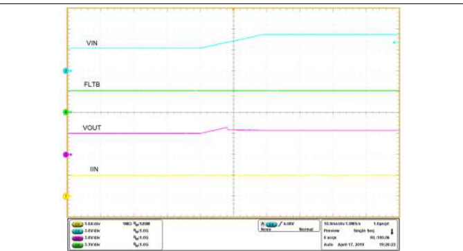
OVCSEL = Shorted to GND, V_{IN} increased from 3 V to 5 V
