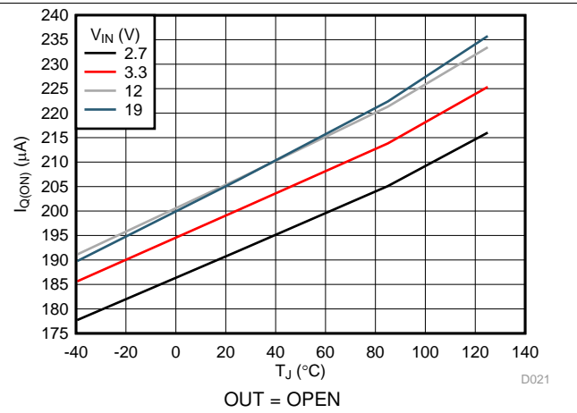
Figure 3. TPS25962x Quiescent Current
