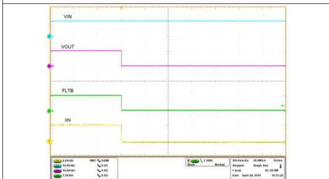
V_{IN} = 12\text{ V} , R_{ILM} = 453\ \Omega , R_{OUT} = 5\ \Omega
