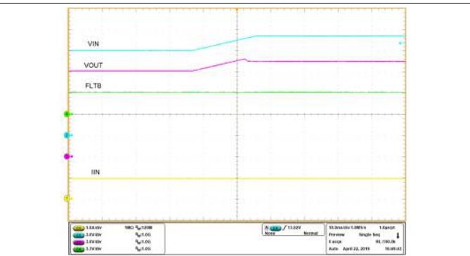
OVCSEL = OPEN, V_{IN} increased from 12 V to 14 V
