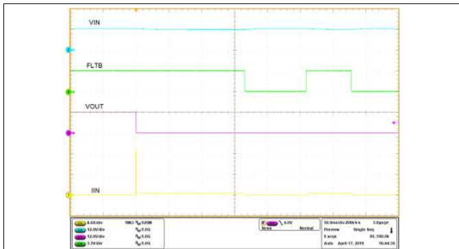
V_{IN} = 12\text{ V} , R_{ILM} = 453\ \Omega
