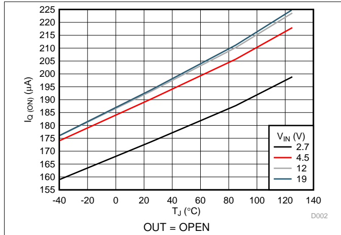
Figure 2. TPS25963x Quiescent Current
