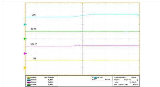
OVCSEL = 400 K \Omega to GND, V_{IN} increased from 5 V to 7 V
