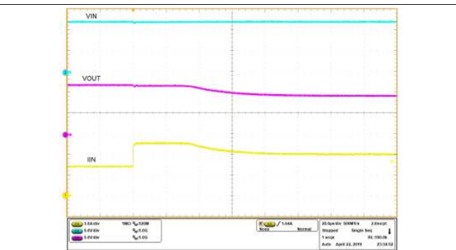
V_{IN} = 12\text{ V} , R_{ILM} = 453\ \Omega , R_{OUT} Varied From 8.33\ \Omega to 4.54\ \Omega
