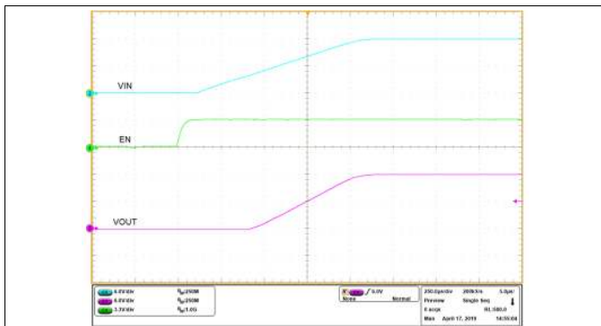
V_{IN} = 12\text{ V} , V_{EN} = 3.3\text{ V}
