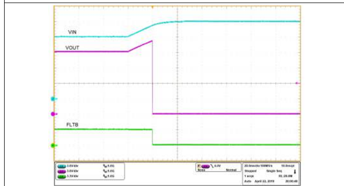
V_{IN} increased from 12 V to 15 V
