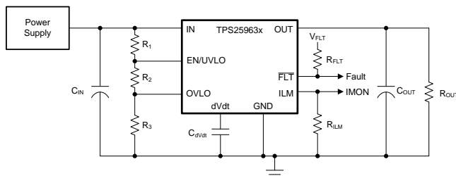
Simplified Schematic
