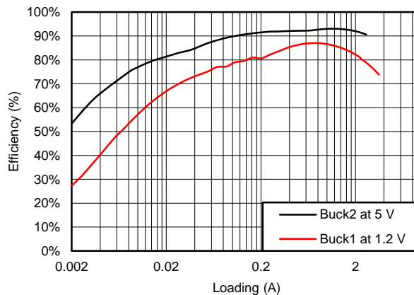
Efficiency, V_{in} = 12\text{ V} , PSM
