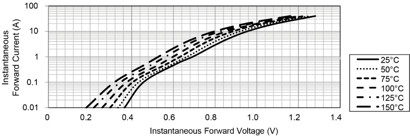
Figure 3. Typical Instantaneous Forward Characteristics
