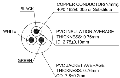
Wire cross section
