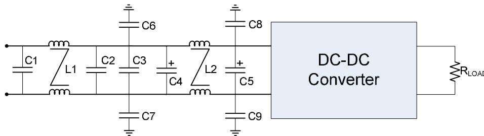
Figure 17. EMI Filter
