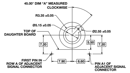
RVPX PIN FOOTPRINT SCALE 4/1
