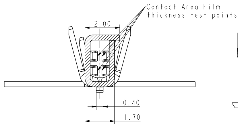
SECTION E-E
