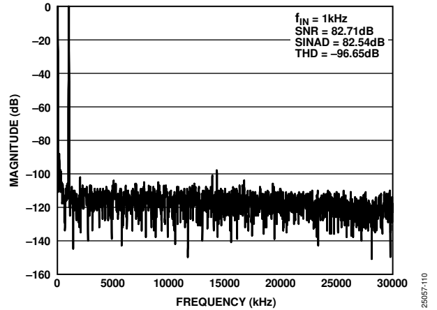
Figure 10. Typical Fast Fourier Transform (FFT)
