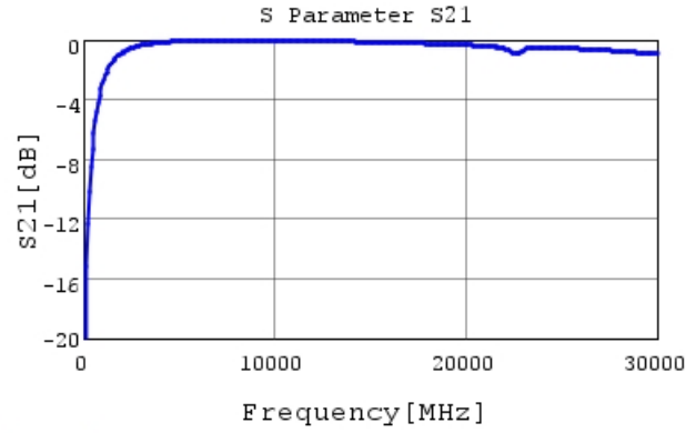
GJM0335C1E1R6CB01 S21 DCOV, 25degC
