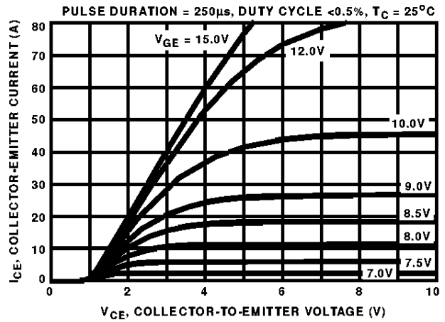
FIGURE 2. SATURATION CHARACTERISTICS
