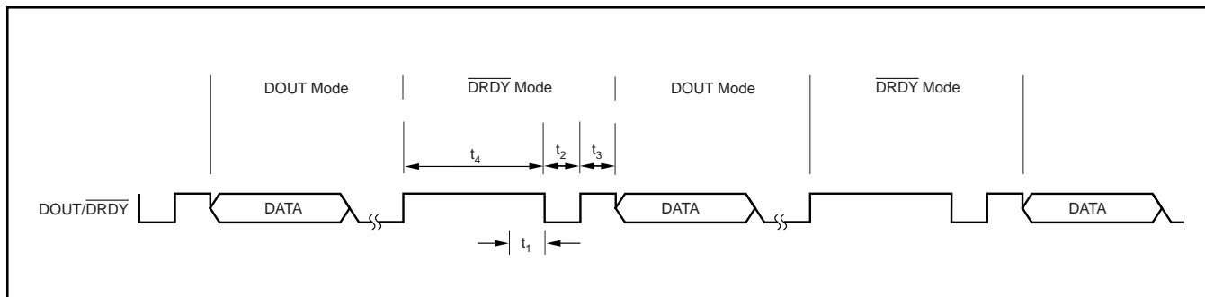
FIGURE 12. DOUT/DRDY Partitioning.
