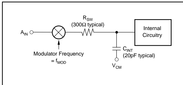
FIGURE 1. Analog-Input Structure.
