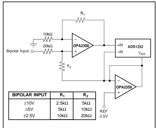
FIGURE 2. Level Shift Circuit for Bipolar Input Ranges.
