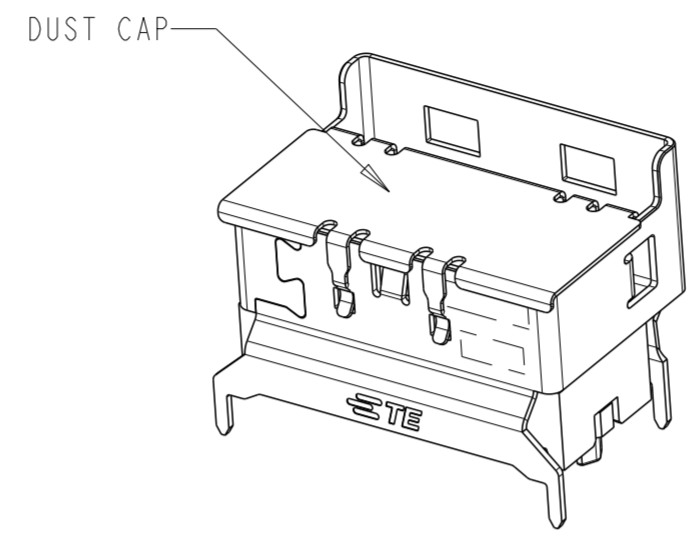
W/ DUST CAP SCALE 4:1
