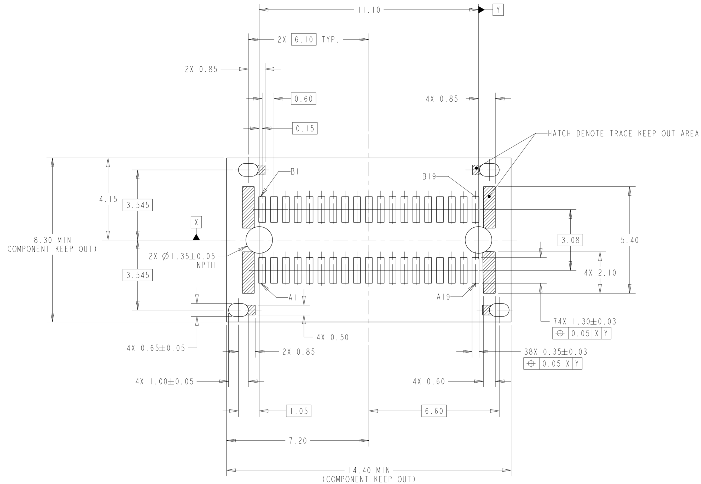
RECOMMENDED PCB LAYOUT AND KEEP OUT AREA TOP VIEW TOLERANCE: ±0.05 SCALE 10:1
