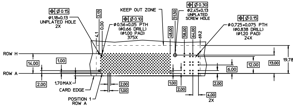
DAUGHTERCARD HOLE PATTERN (CONNECTOR SIDE)
