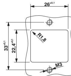
Dimensioned drawing
