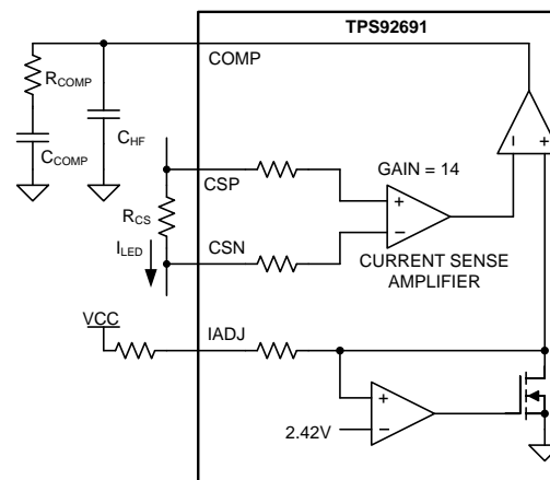
Figure 31. Proportional-Integral Compensation
