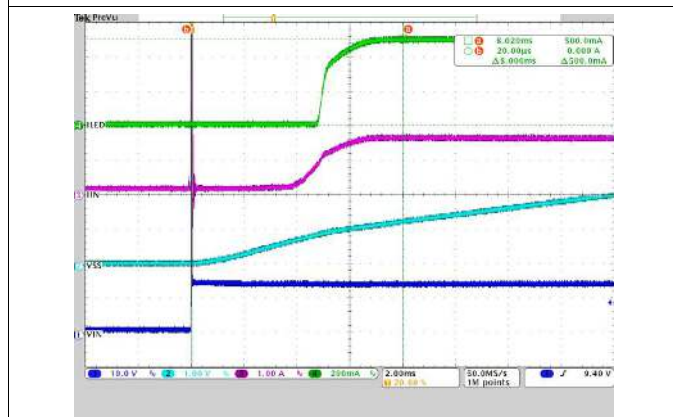
Ch1: Input voltage; Ch2: Soft-start (SS) voltage; Ch3: Input current; Ch4: LED current; Time: 2 ms/div Figure 35. Startup Transient
