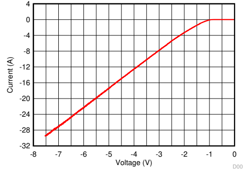
D002_TLP_GND_IO.grf
