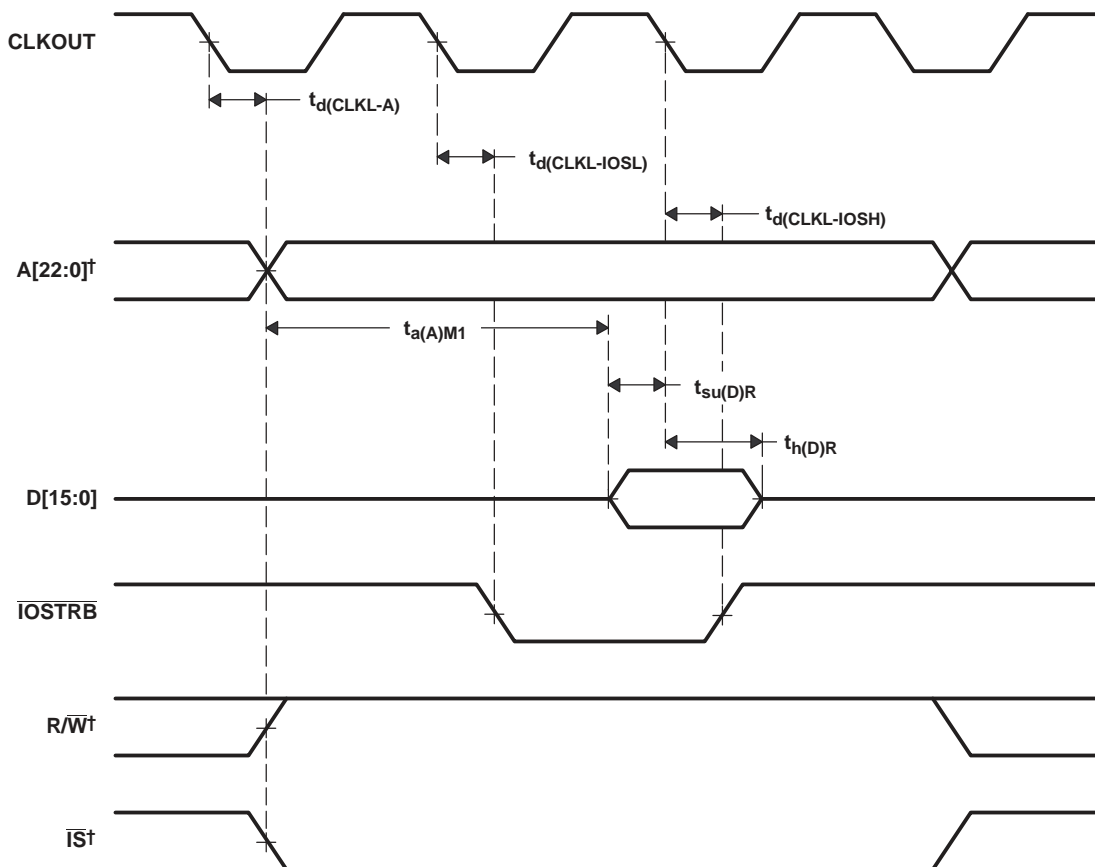
Figure 5-8. Parallel I/O Port Read ( \overline{IOSTRB} = 0 )
