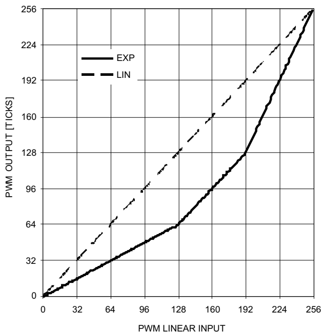
Figure 3. Graph of PWM Output vs. PWM Input
