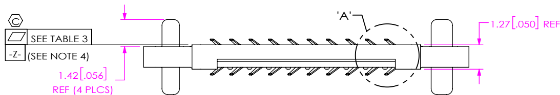
FIG 1 GMI-10-2-1.27-X-10 SHOWN
