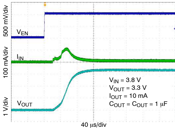
Figure 28. Enable Turn-on Response – V OUT = 3.3 V, C OUT = 1 µF
