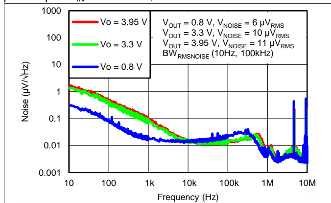
Figure 43. Spectral Noise Density vs Output Voltage
