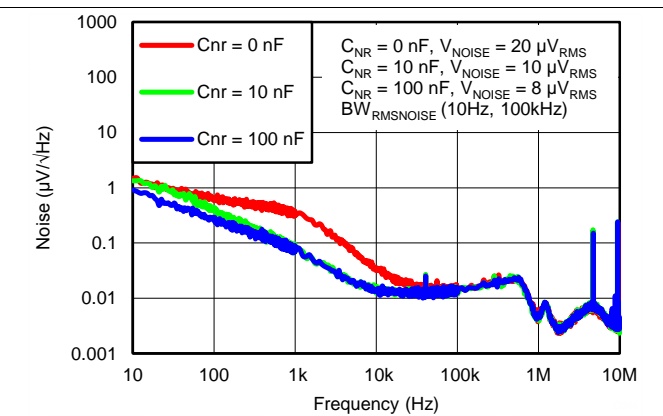
Figure 44. Spectral Noise Density vs C_{NR/SS}
