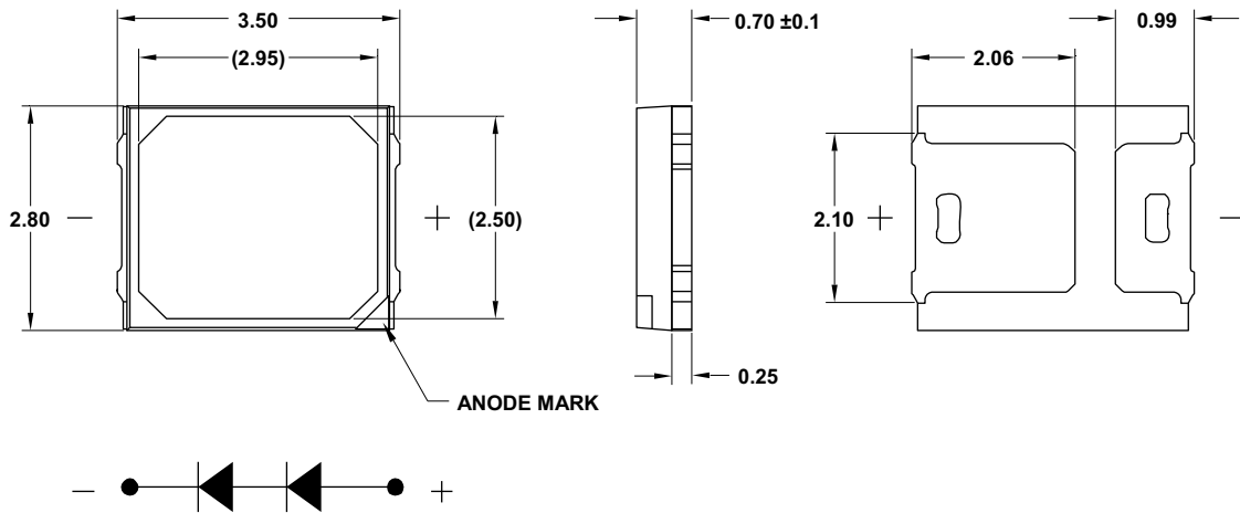
Figure 1: Package Drawing
