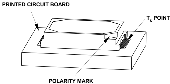
Figure 25: Solder Point Temperature on PCB
