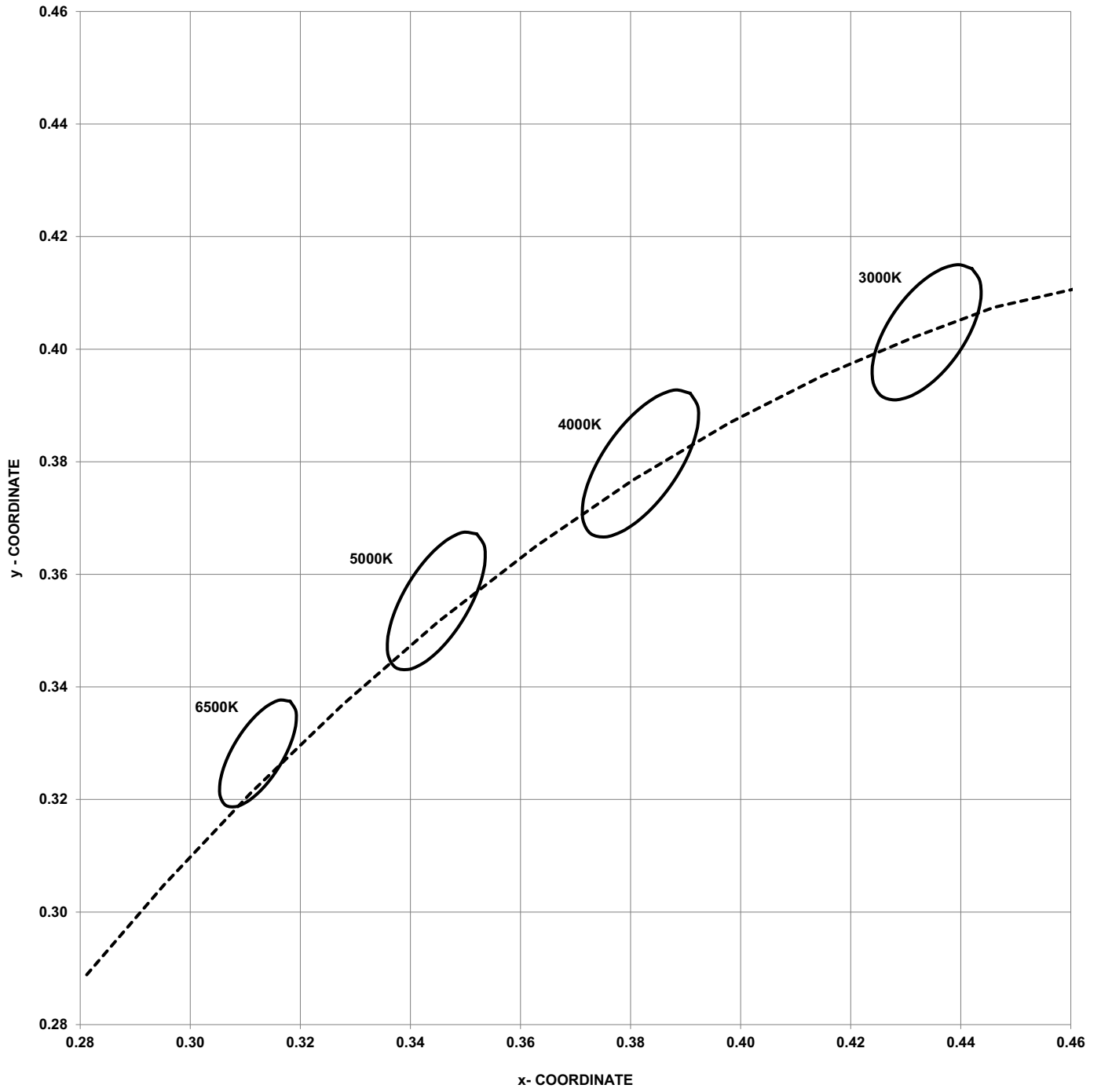
Figure 3: Chromaticity Diagram
