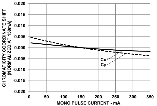
Figure 9: Chromaticity Coordinate Shift vs. Mono Pulse Current – 4000K
