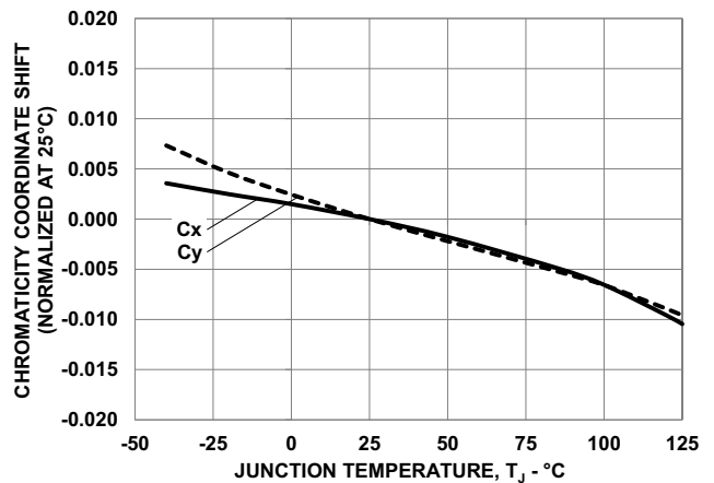
Figure 15: Chromaticity Coordinate Shift vs. Junction Temperature – 4000K
