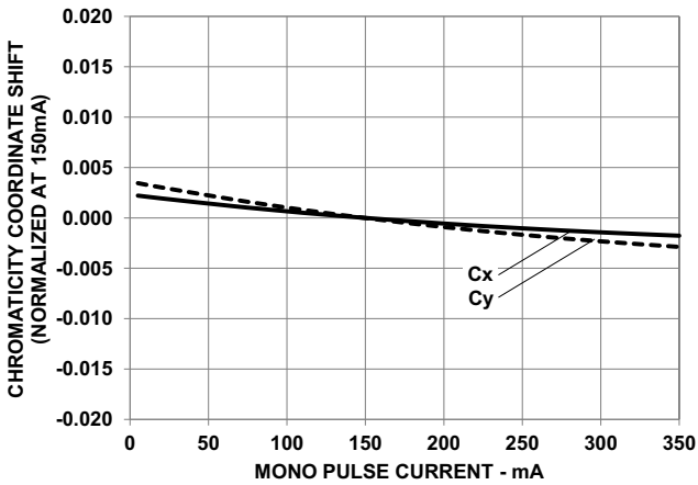
Figure 8: Chromaticity Coordinate Shift vs. Mono Pulse Current – 3000K
