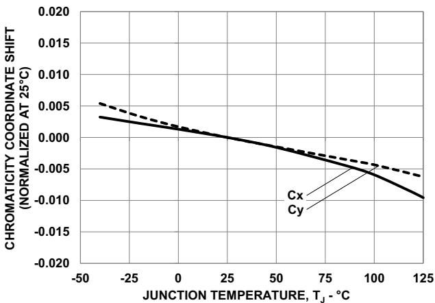
Figure 14: Chromaticity Coordinate Shift vs. Junction Temperature – 3000K
