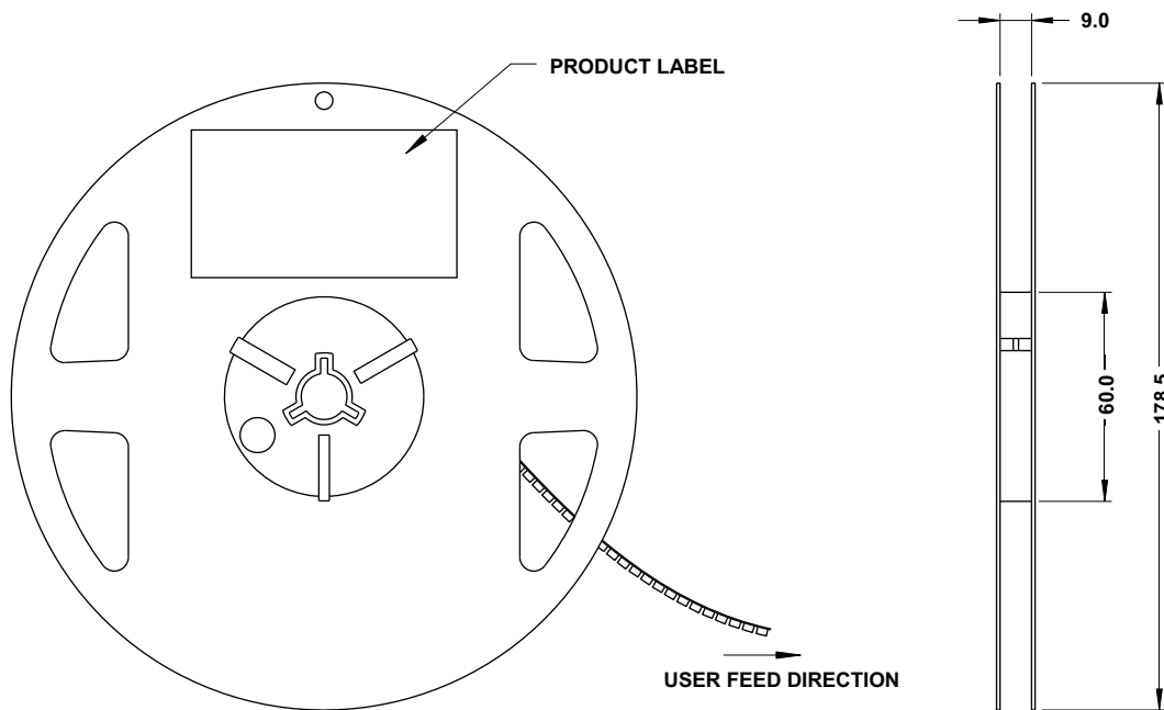
Figure 22: Reel Dimensions
