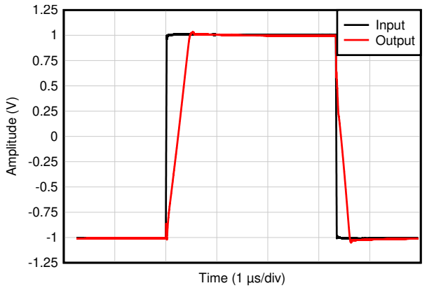
C_L = 20\text{ pF} , Gain = +1, V_{IN} = 2\text{-V step} , R_L = 1\text{ k}\Omega
