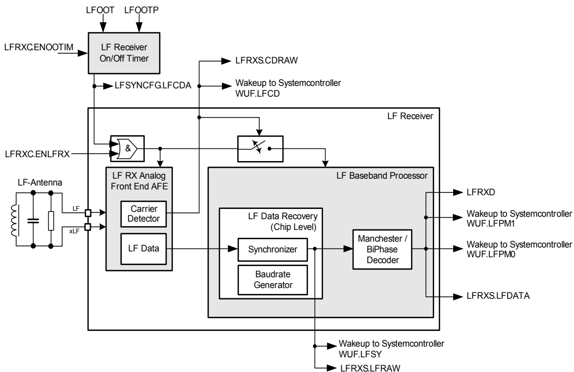
Figure 18 LF Receiver
