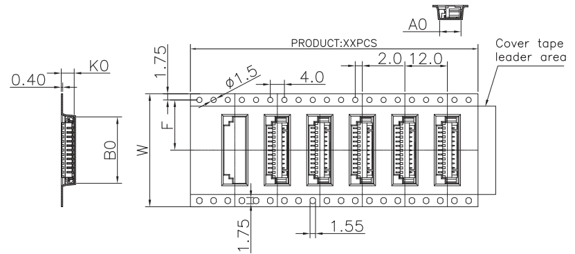
For Reel width (dimension W)32,44,56,72mm ,Double rows hole
