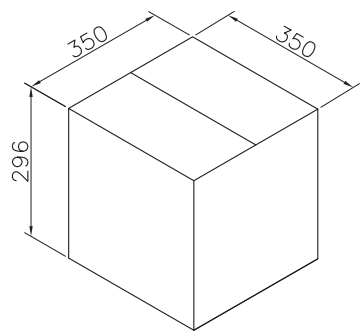
For Reel width (dimension W)32,44,56,72mm ,Double rows hole
