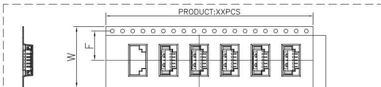
For Reel width (dimension W)16,24mm ,3 & 5PIN ONLY
