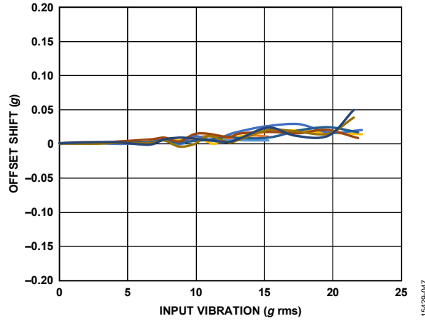
Figure 47. ADXL357 VRE, X-Axis Offset from -1 g, ±40 g Range, X-Axis Orientation = -1 g
