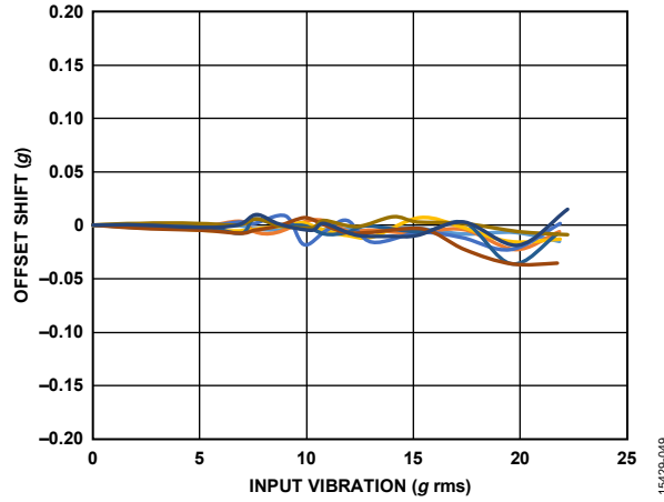
Figure 49. ADXL357 VRE, Z-Axis Offset from +1 g, ±40 g Range, Z-Axis Orientation = +1 g
