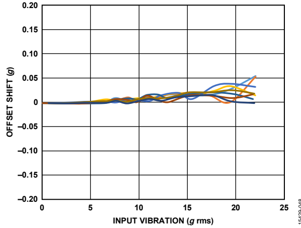
Figure 48. ADXL357 VRE, Y-Axis Offset from -1 g, ±40 g Range, Y-Axis Orientation = -1 g
