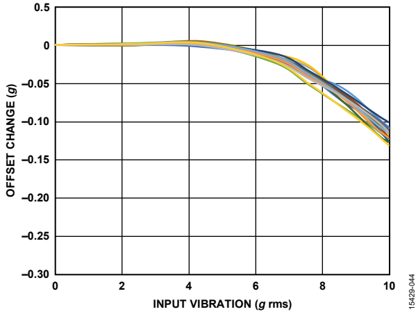
Figure 44. ADXL357 VRE, X-Axis Offset from +1 g, ±10 g Range, X-Axis Orientation = +1 g
