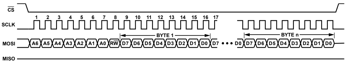
Figure 69. SPI Timing Diagram—Multibyte Write
