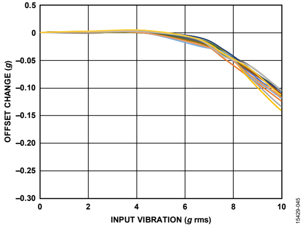
Figure 45. ADXL357 VRE, Y-Axis Offset from +1 g, ±10 g Range, Y-Axis Orientation = +1 g
