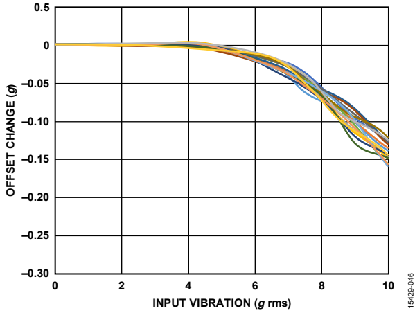
Figure 46. ADXL357 VRE, Z-Axis Offset from +1 g, ±10 g Range, Z-Axis Orientation = +1 g
