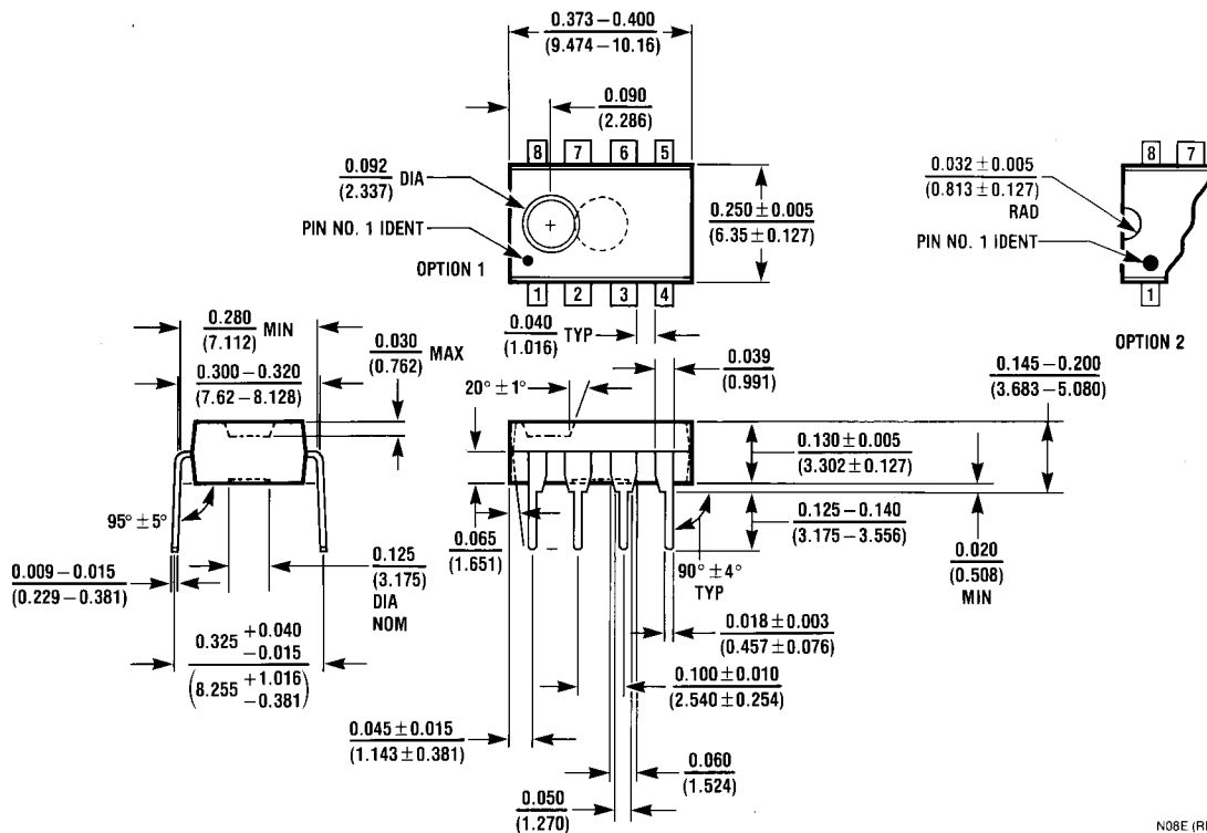
8-Lead (0.300" Wide) Molded Dual-In-Line Package Order Number LMC6442AIN or LMC6442IN or LMC6442INX NS Package Number N08E
