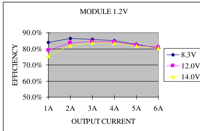
Figure 5. V_o = 1.2 V
