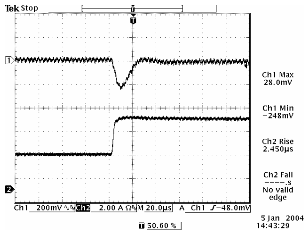
Figure 21. 50% to 100% load step at V_{in} = 12\text{ V} , V_o = 2.5\text{ V}
