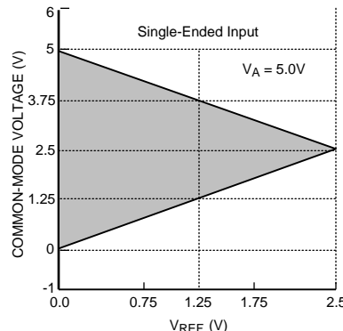
Figure 47. V_{CM} range for single-ended operation
